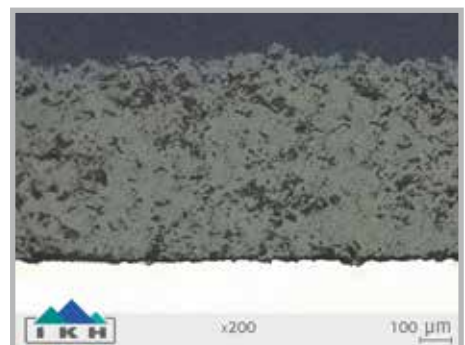
Porosity about 18%
